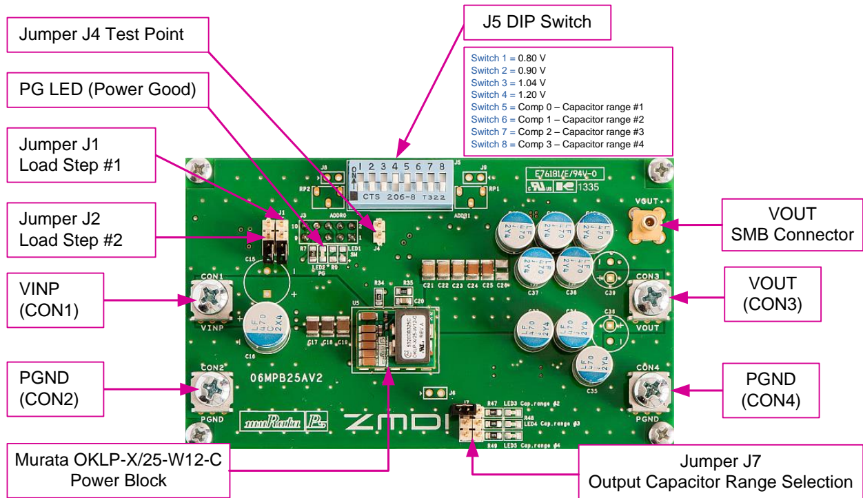
Figure 2.1 ZSPM8725-KIT Evaluation Board (Top Side)
