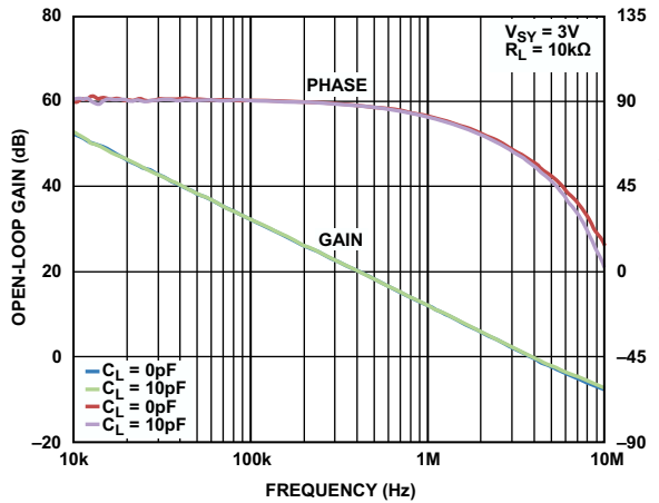
Figure 32. Open-Loop Gain and Phase vs. Frequency
