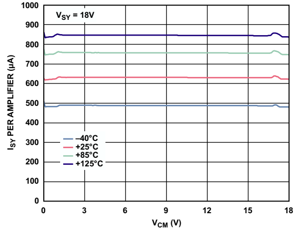
Figure 33. Supply Current vs. Common-Mode Voltage
