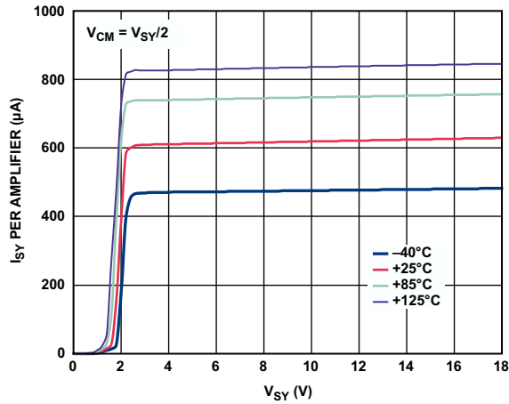
Figure 31. Supply Current vs. Supply Voltage
