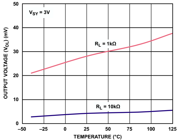
Figure 26. Output Voltage ( V_{OL} ) vs. Temperature
