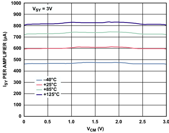
Figure 30. Supply Current vs. Common-Mode Voltage
