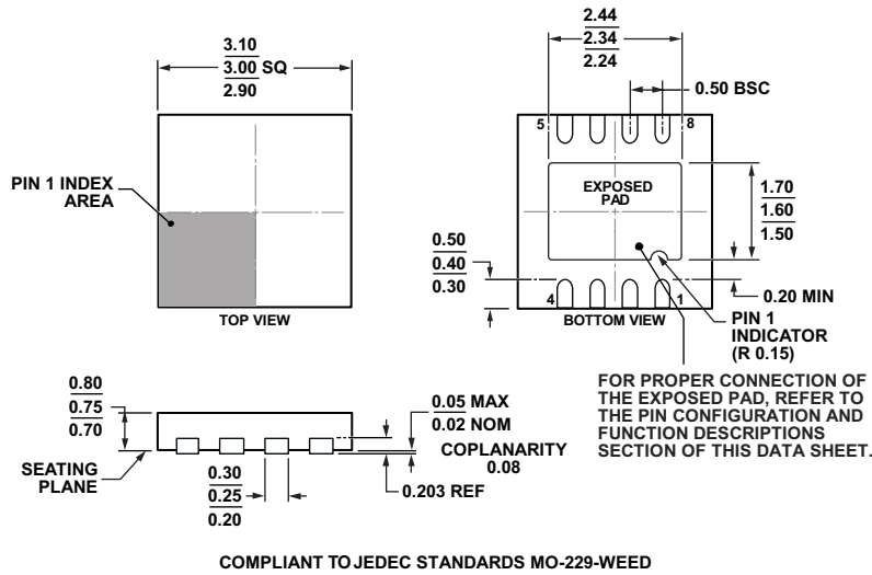
Figure 92. 8-Lead Lead Frame Chip Scale Package [LFCSP_WD] 3 mm x 3 mm Body, Very Very Thin, Dual Lead (CP-8-11)
