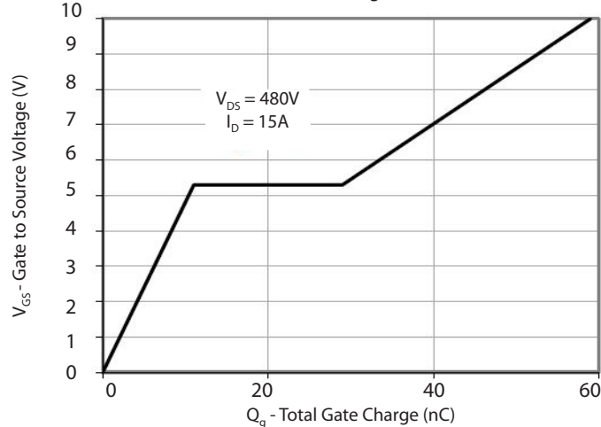
Gate Charge
