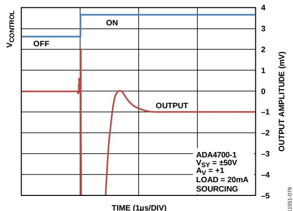
Figure 17. Output Current Transient Settling Time (Sourcing), V_{SY} = \pm 50\text{ V} , Refer to Figure 56 for the Test Circuit
