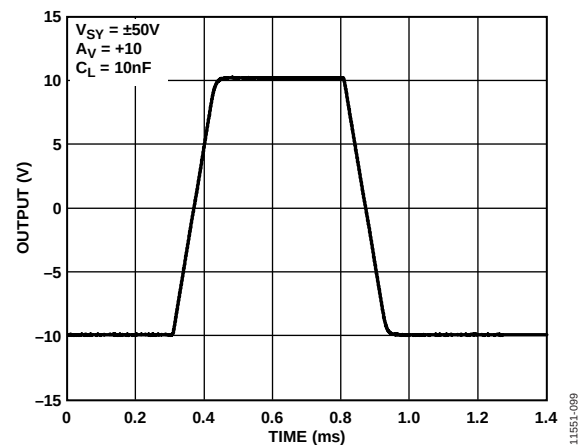
Figure 65. Results from Snubber Network with Higher Gains, C_L = 10 \text{ nF}
