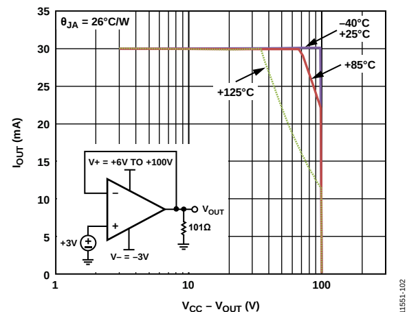
Figure 59. Safe Operating Area with \theta_{JA} = 26^\circ\text{C/W}
