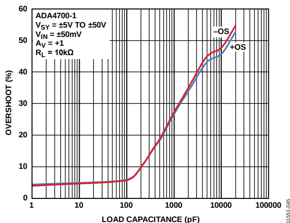
Figure 30. Small Signal Overshoot vs. Load Capacitance, V_{SY} = \pm 5\text{ V to } \pm 50\text{ V}
