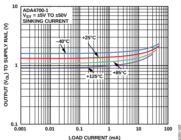
Figure 19. Output Voltage ( V_{OL} ) to Supply Rail vs. Load Current, V_{SY} = \pm 5\text{ V to } \pm 50\text{ V}
