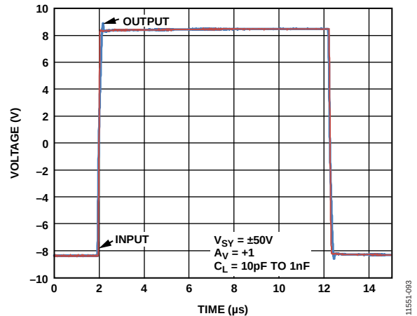
Figure 64. Results from Snubber Network with A_V = +1 and C_L = 10 \text{ pF} to 1 \text{ nF}
