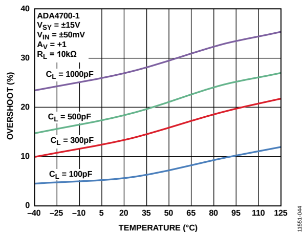
Figure 29. Small Signal Overshoot vs. Temperature for Various Capacitance Loads, V_{SY} = \pm 15\text{ V}
