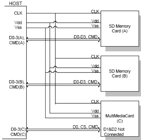
Figure 4-2: mcryptoSD Card system bus Topology
