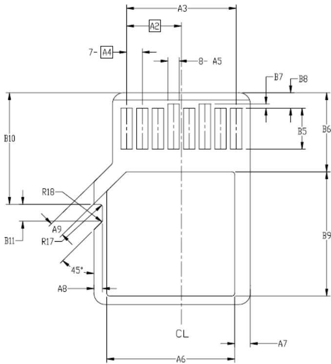
Figure 42-11: Dimensions of microSD (Bottom View)
