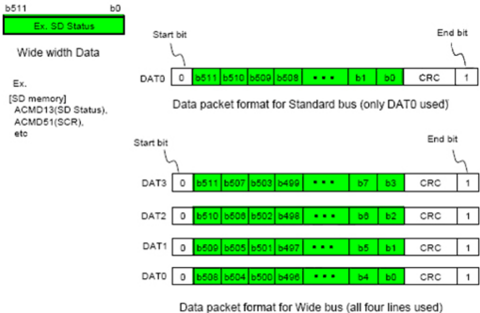
Figure 6-7: Data packet format - Wide width data
