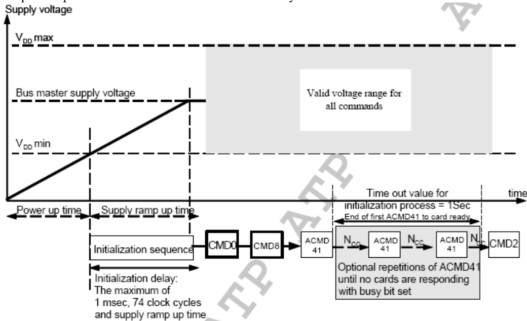
Figure 4-4: Power-up diagram
