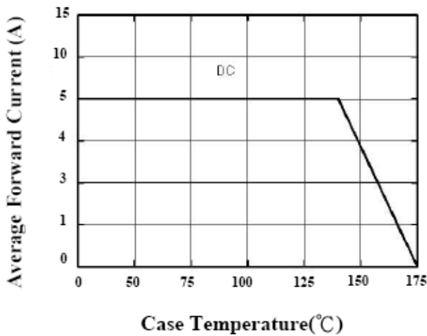
Fig.1- Forward Current
