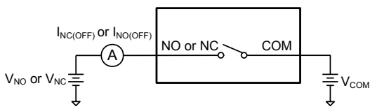
Test Circuit 2. Off Leakage
