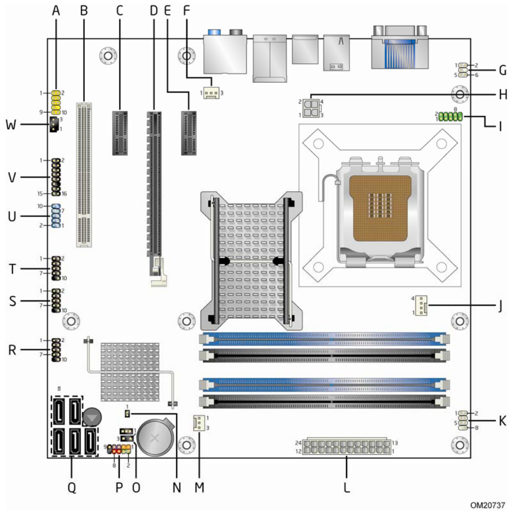
Figure 10. Component-side Connectors and Headers
