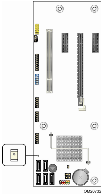
Figure 7. Location of the Standby Power Indicator LED
