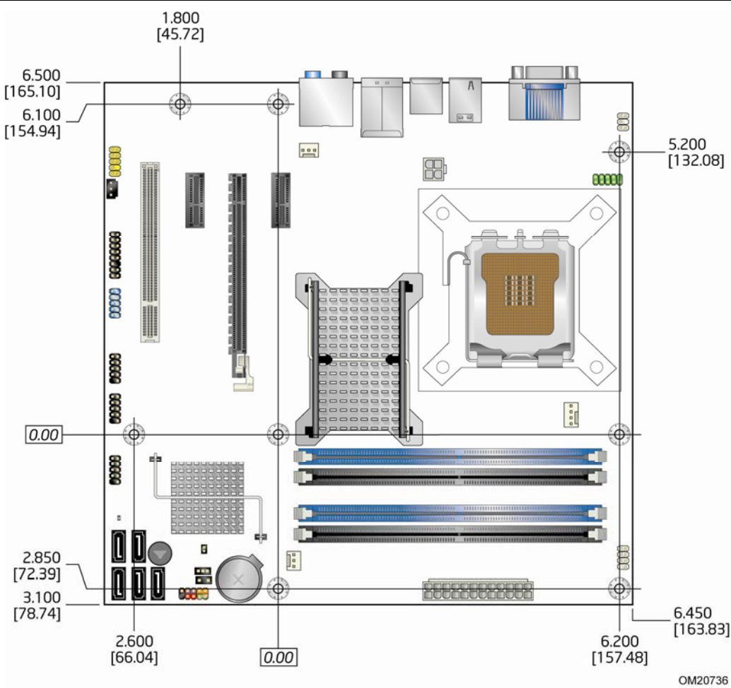
Figure 15. Board Dimensions
