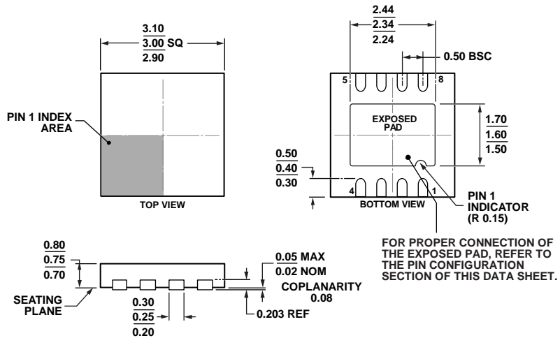
Figure 80. 8-Lead Lead Frame Chip Scale Package [LFCS_P_WD] 3 mm x 3 mm Body, Very Very Thin, Dual Lead (CP-8-11)
