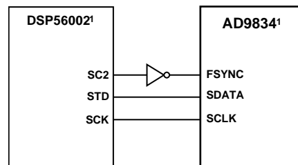
Figure 38. DSP56002 to AD9834 Interface
