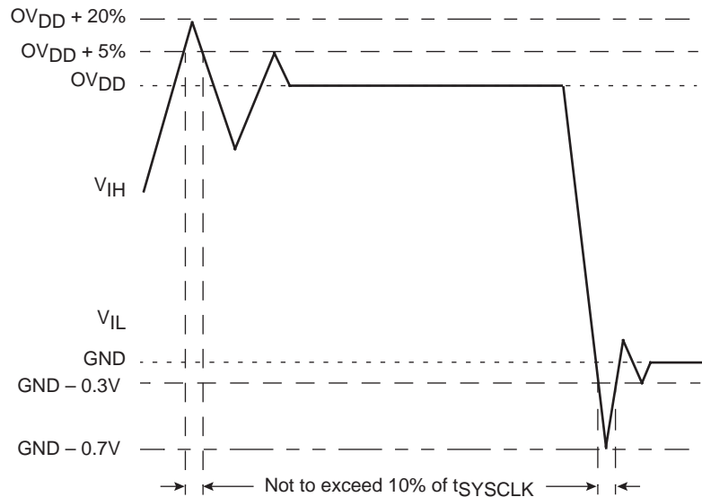
Figure 3. Overshoot/Undershoot Voltage
