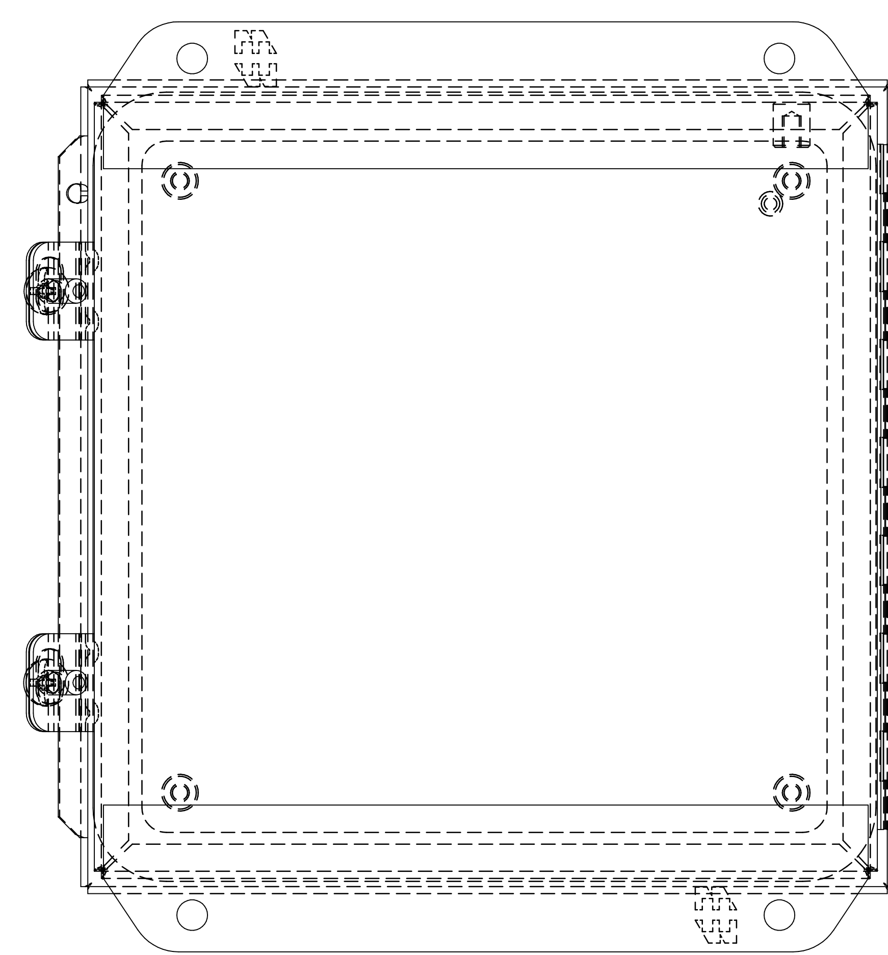
BACK VIEW
