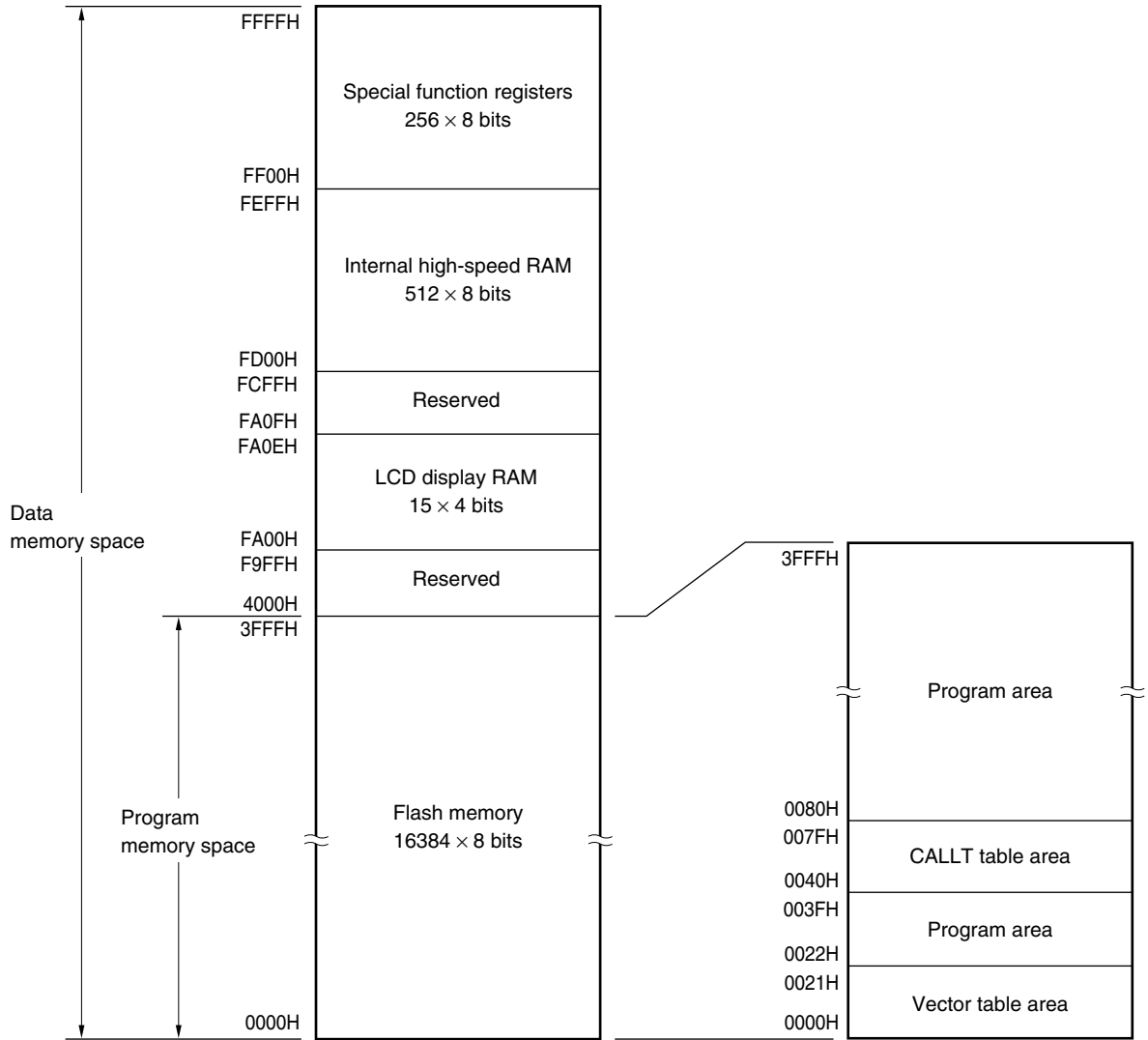
Figure 3-6. Memory Map ( \mu PD78F9456)
