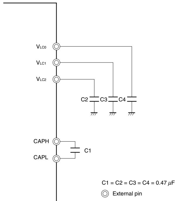
Figure 13-14. Example of Connecting Pins for LCD Driver
