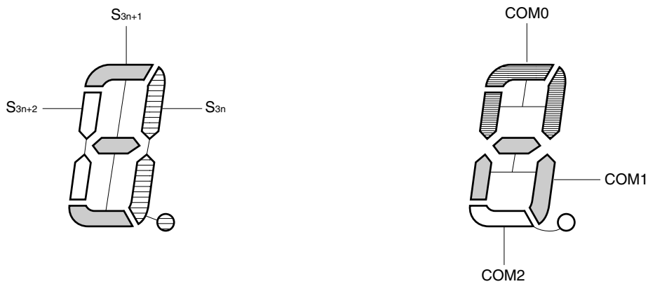
Figure 13-8. Three-Time Slot LCD Display Pattern and Electrode Connections
