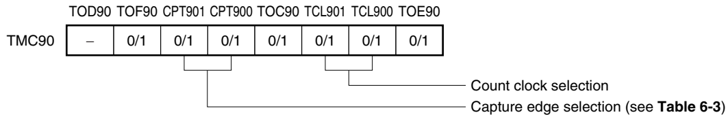
Figure 6-9. Settings of 16-Bit Timer Mode Control Register 90 for Capture Operation
