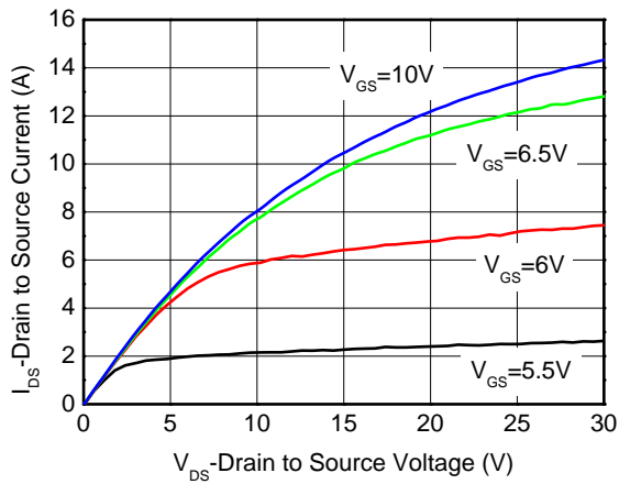
Output characteristics
