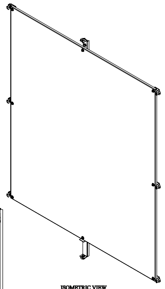
ISOMETRIC VIEW
