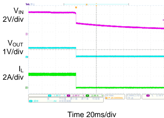
Power off Waveform ( V_{IN}=V_{CC}=5V , V_{OUT}=1V , I_{OUT}=3A )
