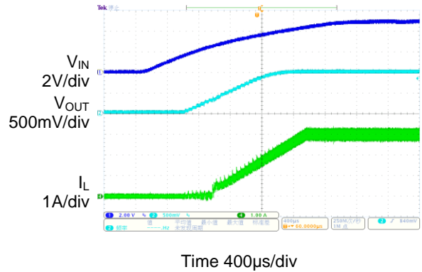
Power on Waveform ( V_{IN}=V_{CC}=5V , V_{OUT}=1V , I_{OUT}=3A )
