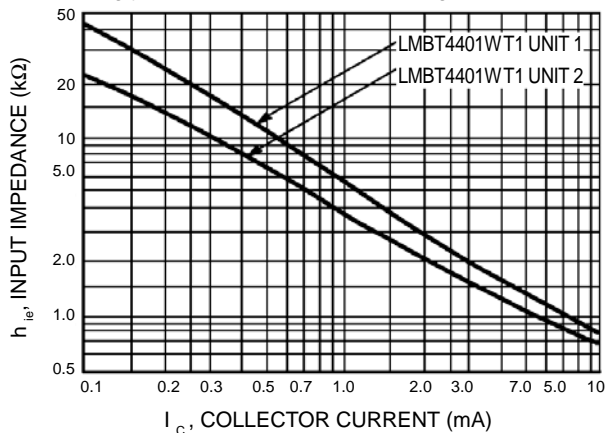
Figure 12. Input Impedance
