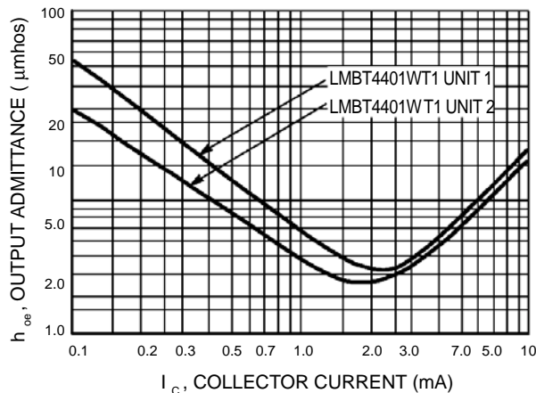
Figure 14. Output Admittance
