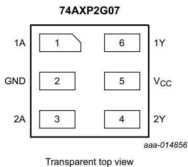
Fig 4. Pin configuration SOT886, SOT1115 and SOT1202
