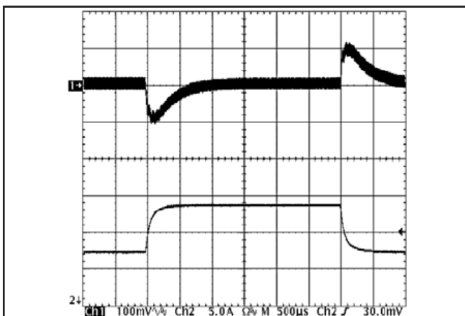
Figure 11: Output voltage response to step-change in load current (50%-75%-50% of I_{max} ; dI/dt = 0.1A/\mu s ). Load cap: 10µF, 100 mΩ ESR tantalum capacitor and 1µF ceramic capacitor. Top trace: V_{out} (100mV/div), Bottom trace: I_{out} (5A/div).
