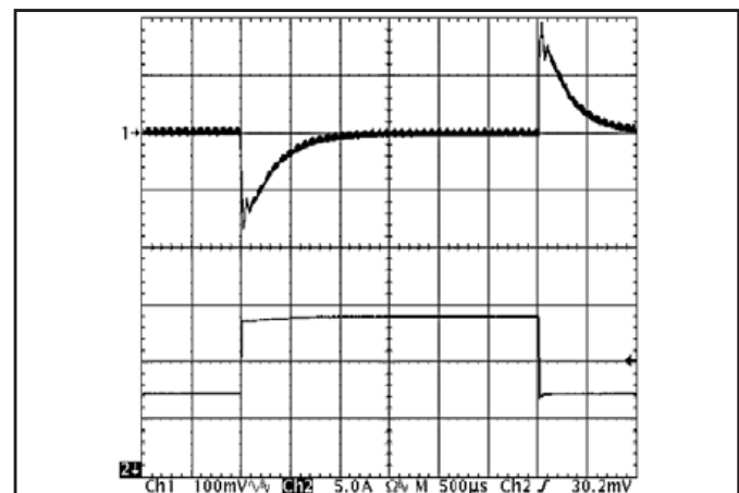
Figure 12: Output voltage response to step-change in load current (50%-75%-50% of I_{max} ; dI/dt = 5A/\mu s ). Load cap: 470µF, 30 mΩ ESR tantalum capacitor and 1µF ceramic capacitor. Top trace: V_{out} (100mV/div), Bottom trace: I_{out} (5A/div).
