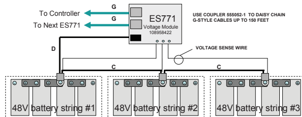
Temperature/Voltage Measurement
