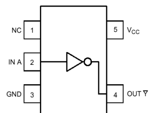
Figure 1. Pinout (Top View)
