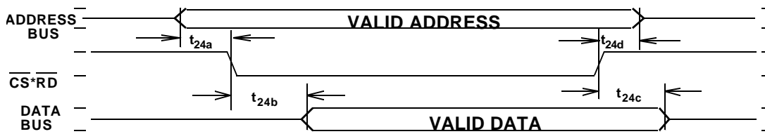
Figure 25. Detailed Timing - RTMP DMA Write Cycle
