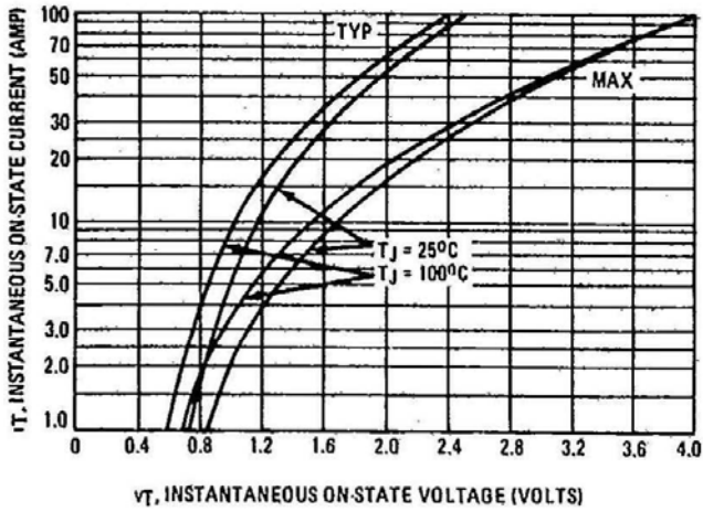
FIGURE 8 – FORWARD VOLTAGE
