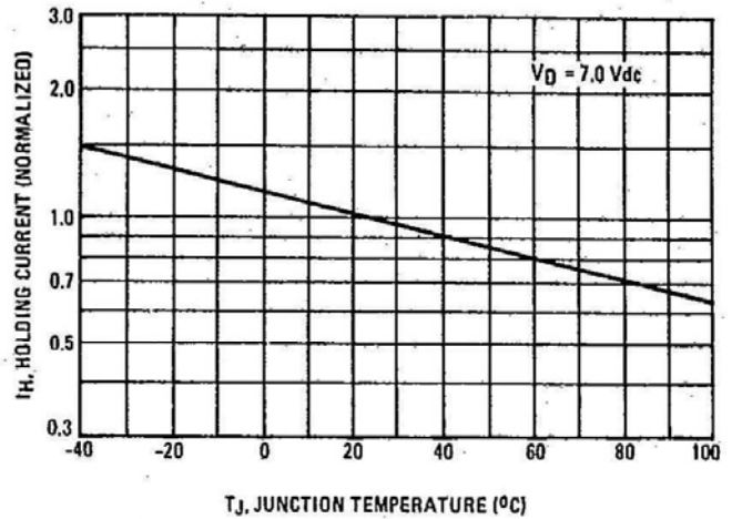
FIGURE 9 – HOLDING CURRENT
