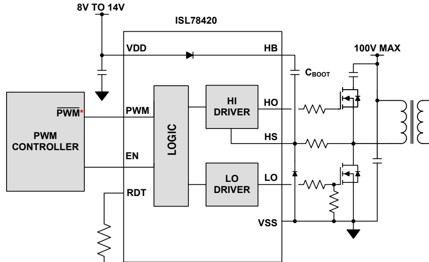
FIGURE 22. TYPICAL ACTIVE CLAMP FORWARD APPLICATION
