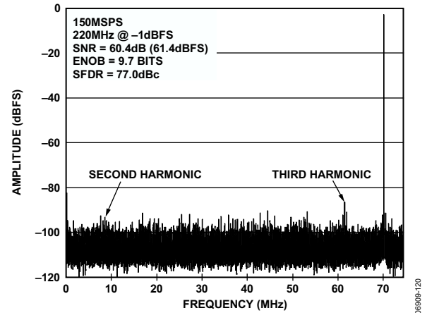
Figure 20. AD9600-150 Single-Tone FFT with f_{IN} = 220 MHz
