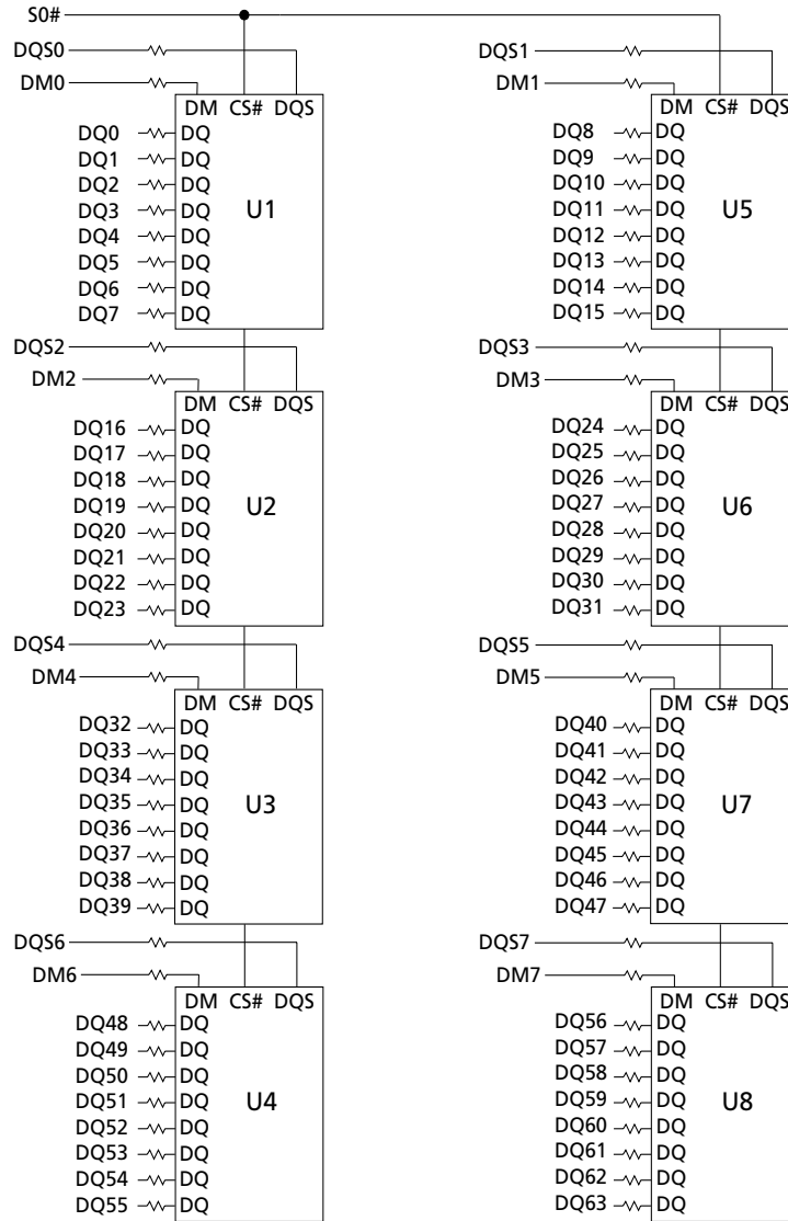
Figure 3: Functional Block Diagram
