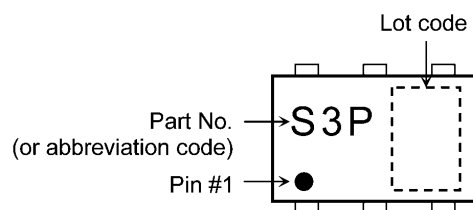
Fig. 7.1 Marking
