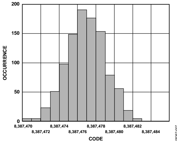
Figure 8. Noise Distribution Histogram ( V_{REF} = AV_{DD} = 5\text{ V} , Output Data Rate = 4.7 Hz, Gain = 128, Chop Disabled, \text{Sinc}^4 Filter)
