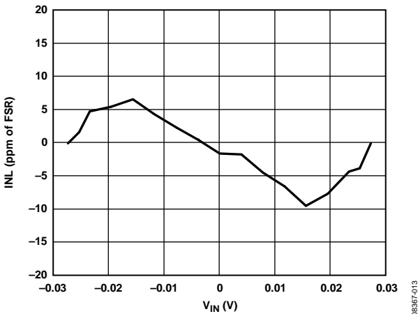
Figure 14. INL (Gain = 128)
