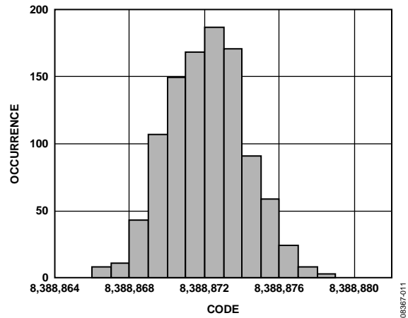
Figure 12. Noise Distribution Histogram ( V_{REF} = AV_{DD} = 5\text{ V} , Output Data Rate = 42.1 Hz ( FS[9:0] = 6 , Average by 16), Gain = 1, Chop Disabled, \text{Sinc}^4 Filter)
