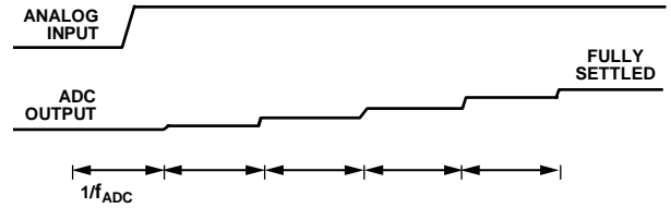
Figure 30. Asynchronous Step Change in Analog Input
