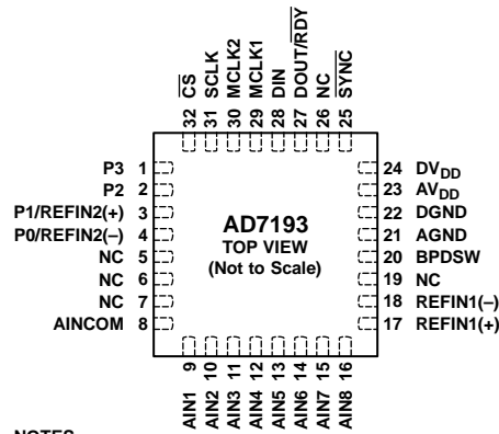
Figure 6. 32-Lead LFCSP Pin Configuration
