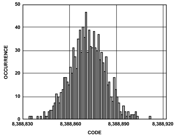
Figure 10. Noise Distribution Histogram ( V_{REF} = AV_{DD} = 5\text{ V} , Output Data Rate = 2400 Hz, Gain = 1, Chop Disabled, \text{Sinc}^4 Filter)
