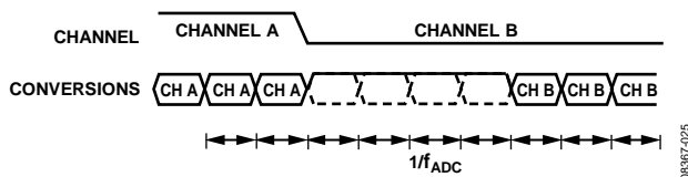
Figure 29. Sinc 4 Channel Change
