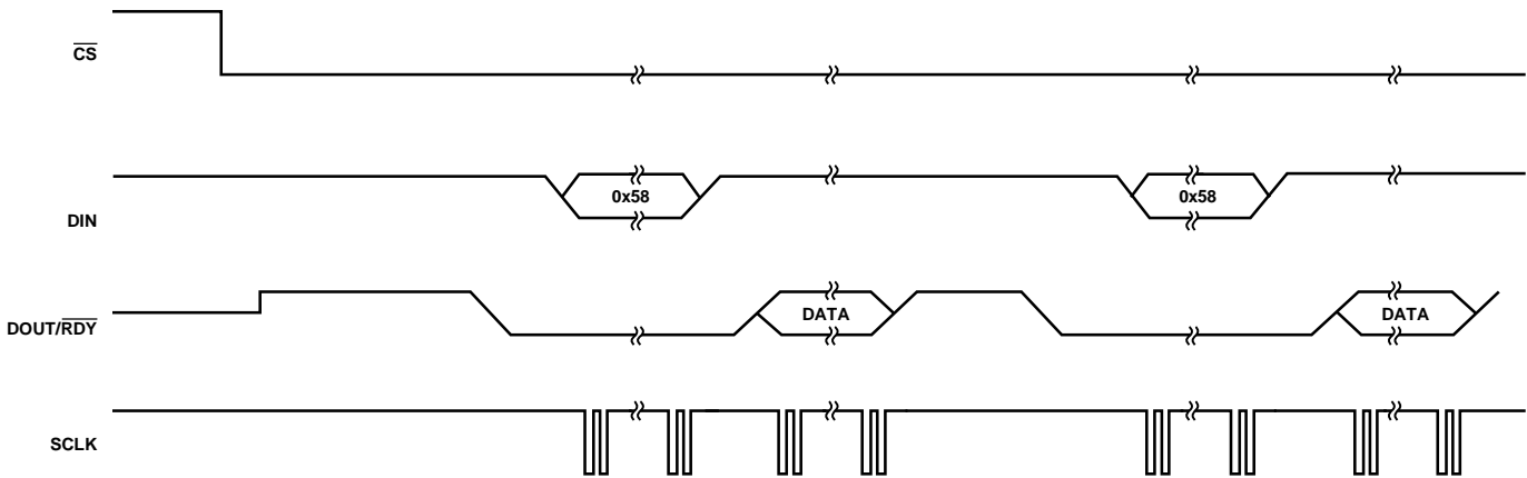
Figure 26. Continuous Conversion
