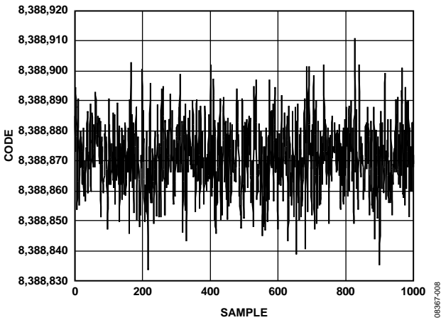
Figure 9. Noise ( V_{REF} = AV_{DD} = 5\text{ V} , Output Data Rate = 2400 Hz, Gain = 1, Chop Disabled, \text{Sinc}^4 Filter)
