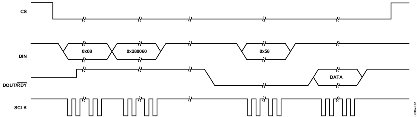
Figure 25. Single Conversion
