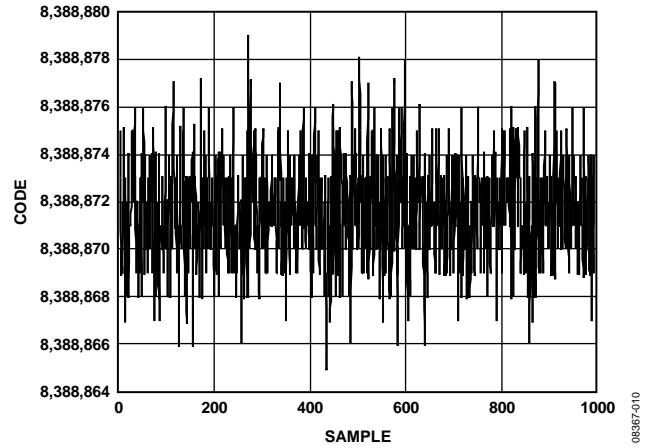
Figure 11. Noise ( V_{REF} = AV_{DD} = 5\text{ V} , Output Data Rate = 42.1 Hz ( FS[9:0] = 6 , Average by 16), Gain = 1, Chop Disabled, \text{Sinc}^4 Filter)
