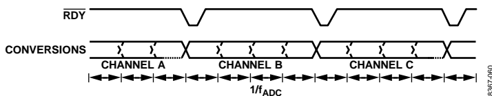
Figure 24. Channel Sequencer
