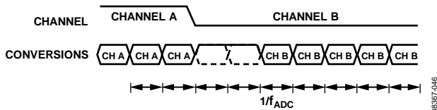
Figure 50. Channel Change (Sinc 3 Chop Enable)
