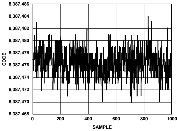
Figure 7. Noise ( V_{REF} = AV_{DD} = 5\text{ V} , Output Data Rate = 4.7 Hz, Gain = 128, Chop Disabled, \text{Sinc}^4 Filter)
