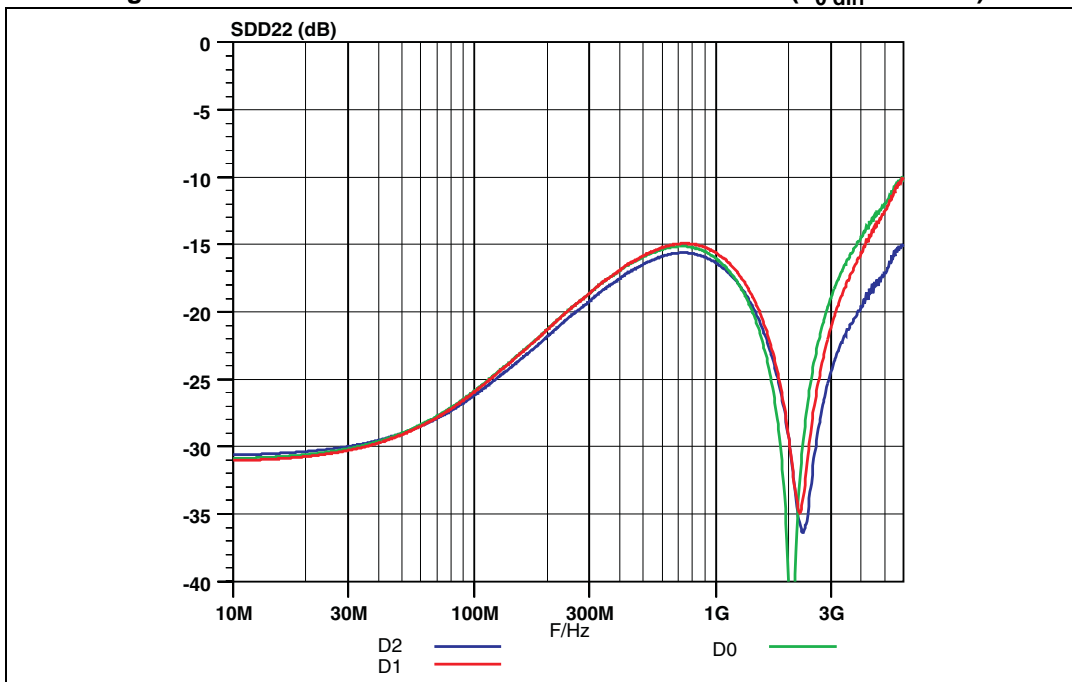
Figure 6. SDD22 differential attenuation measurement ( Z_{0\text{ diff}} = 100 \Omega )
