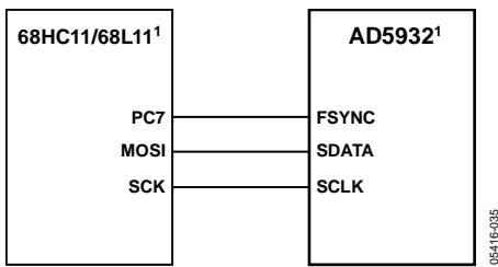
Figure 35. 68HC11/68L11 to AD5932 Interface
