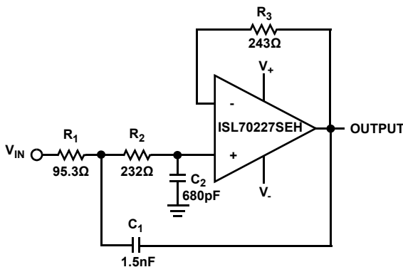
SALLEN-KEY LOW PASS FILTER (1MHz)
