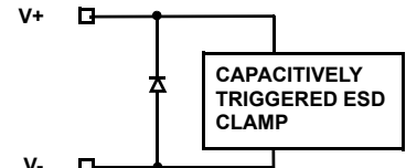
CIRCUIT 3
