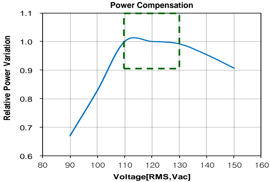
Fig 4. Relative Power Variation vs. Voltage at T_a = 25^\circ\text{C} , 120V
