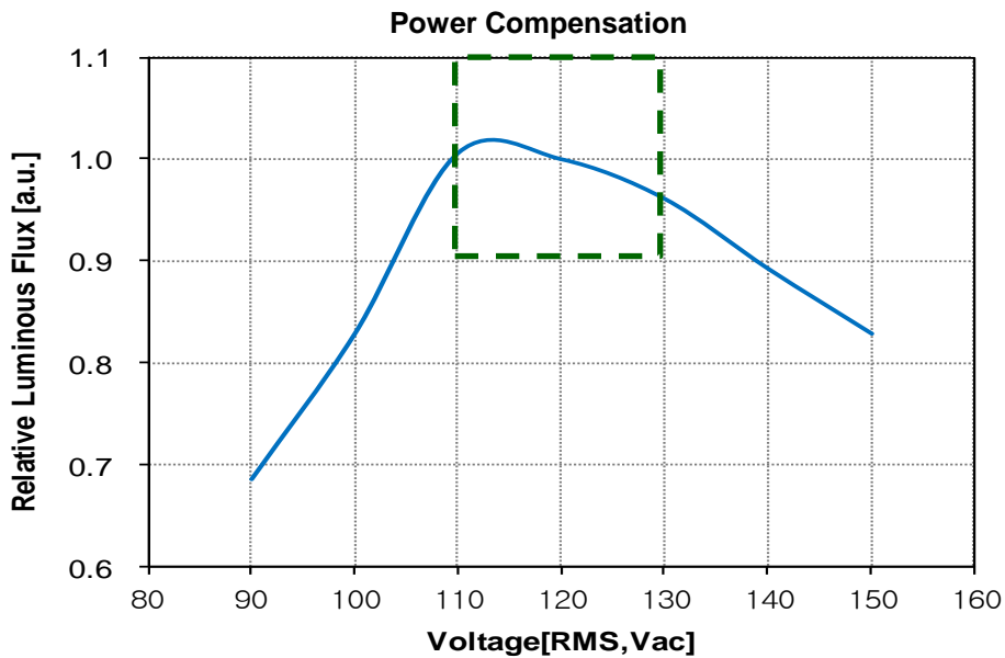
Fig 5. Relative Luminous Flux vs. Voltage at T_a = 25^\circ\text{C} , 120V
