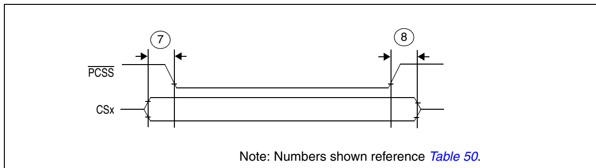
Figure 32. DSPI PCS strobe ( \overline{PCSS} ) timing
