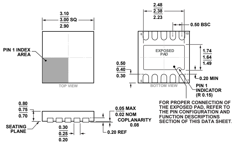
Figure 45. 10-Lead Lead Frame Chip Scale Package [LFCSP_WD] 3 mm x 3 mm, Very Very Thin, Dual Lead (CP-10-9) Dimensions shown in millimeters
