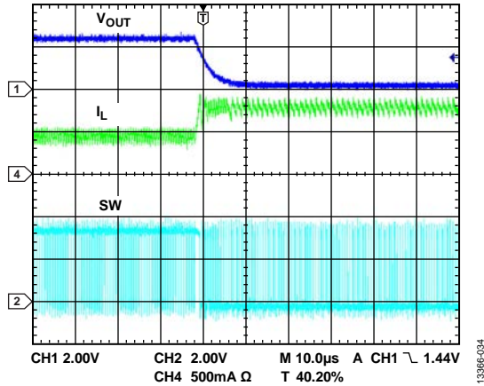
Figure 34. Output Short Protection ( I_L is the Inductor Current)
