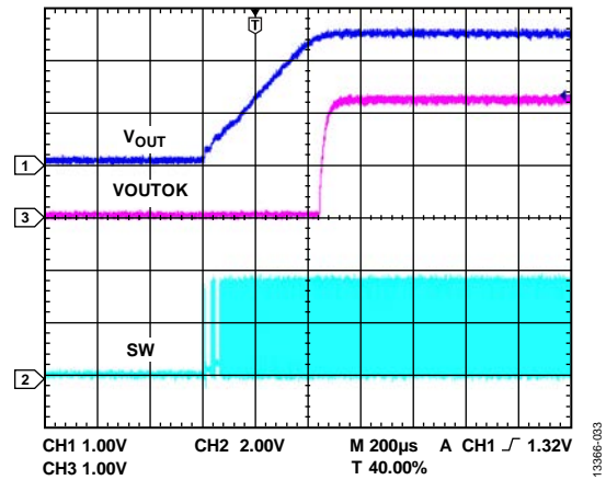
Figure 33. VOUTOK Function
