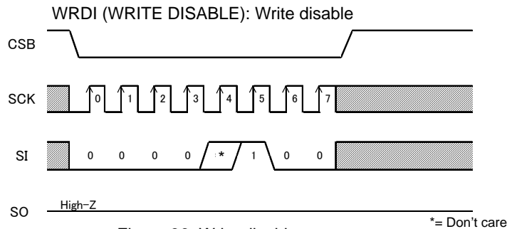
Figure 36. Write disable
