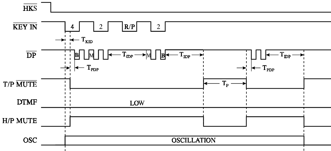
Figure 4. Pause Function
