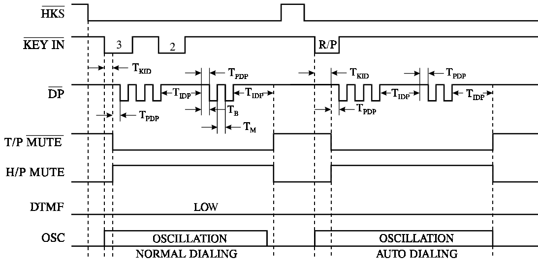
Figure 1. Pulse Mode
