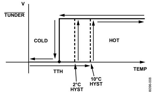
Figure 17. ADT6503 \overline{TUNDER} Transfer Function
