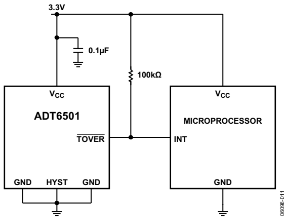
Figure 20. Microprocessor Alarm
