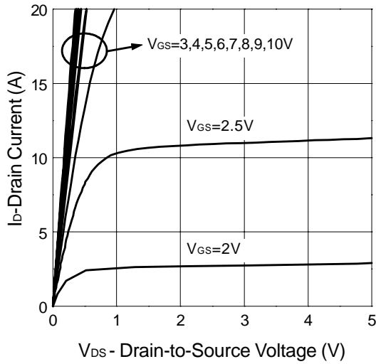
Output Characteristics
