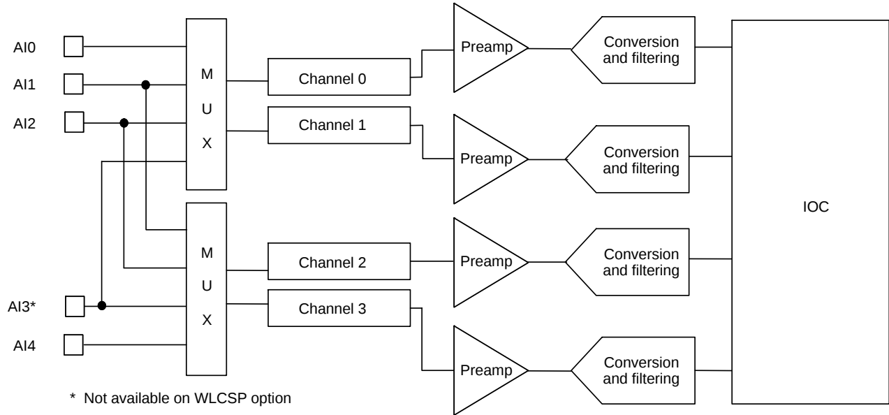
Figure 8. Input Stage
