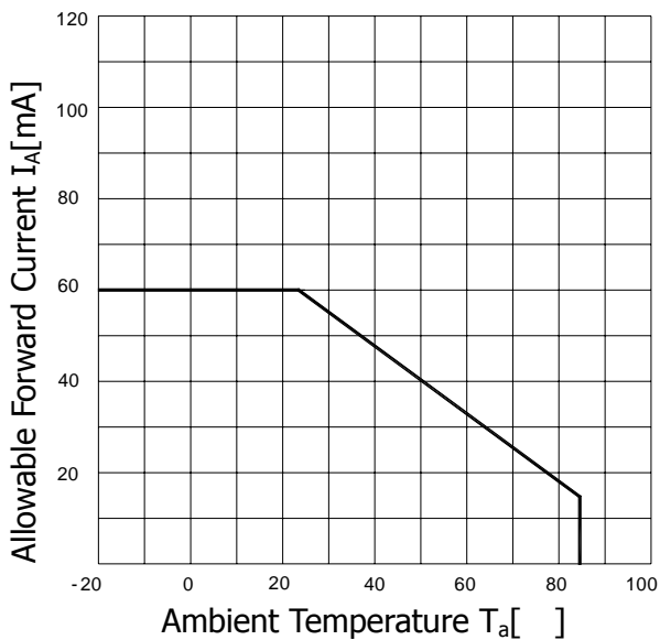
(3) Ambient Temperature vs. Allowable Forward Current
