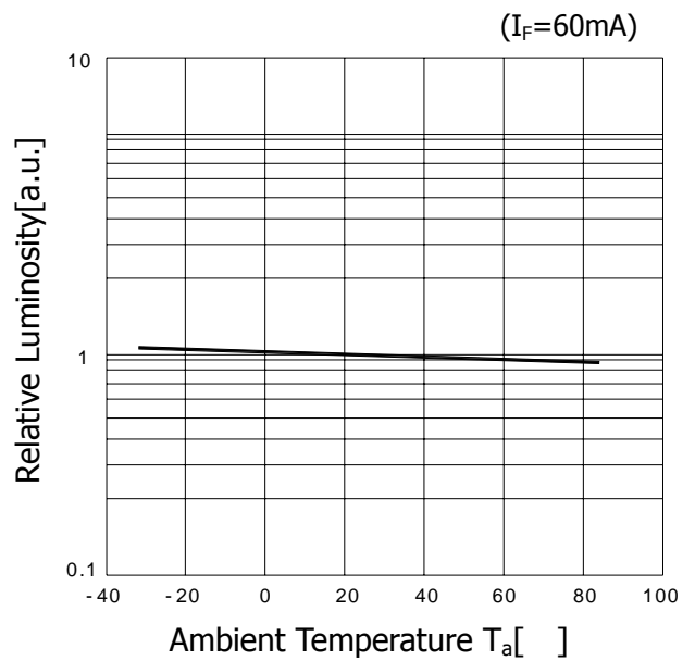
(4) Ambient Temperature vs. Relative Luminosity
