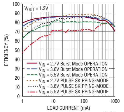
1A Buck Regulators, Efficiency vs Load
