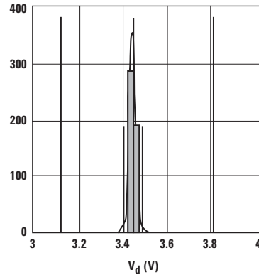
Figure 2. V_d distribution @ 15 mA. LSL = 3.1, Nominal = 3.4, USL = 3.8
