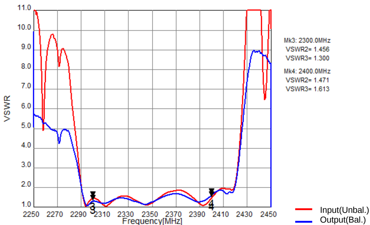
Fig.10 VSWR (Filter2)
