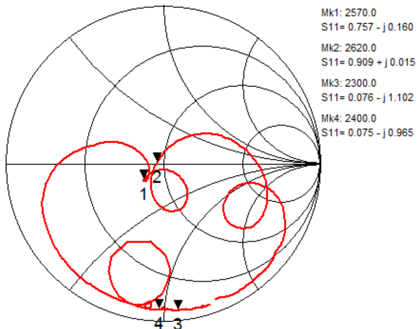
Fig. 5 Input Impedance (Unbalanced) (Filter1)
