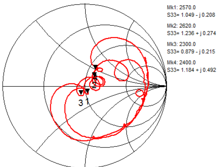
Fig. 5 Input Impedance (Unbalanced) (Filter1)
