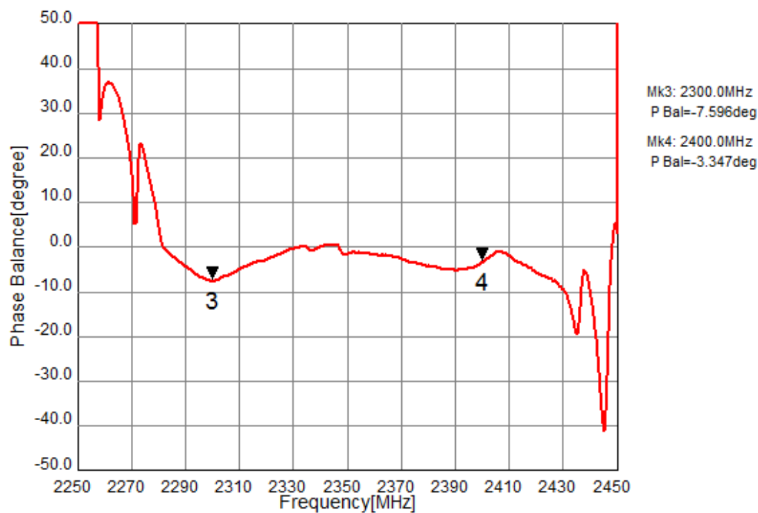
Fig.16 Phase Balanced (Filter2)
