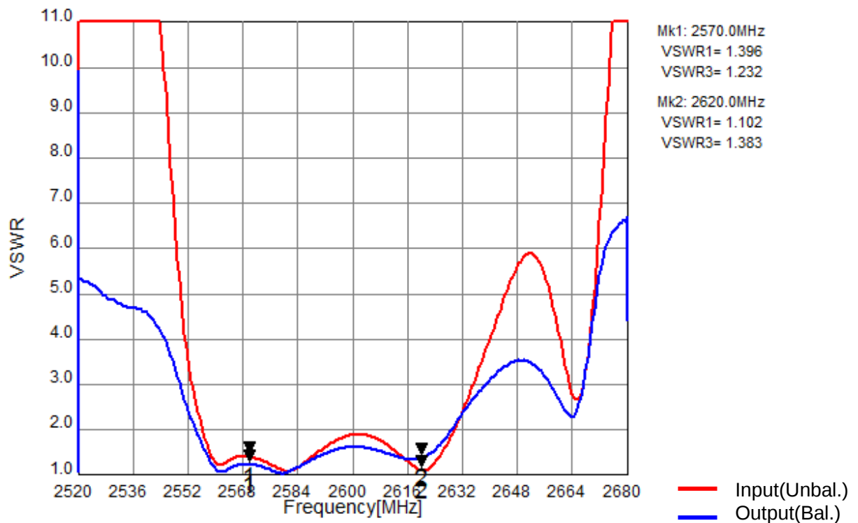
Fig.2 VSWR (Filter1)
