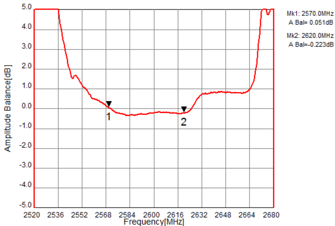
Fig. 7 Amplitude Balanced (Filter1)
