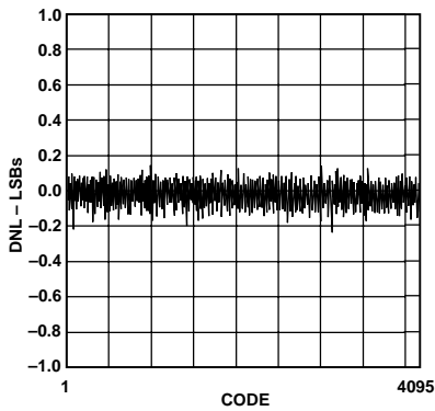
Figure 20. Typical DNL
