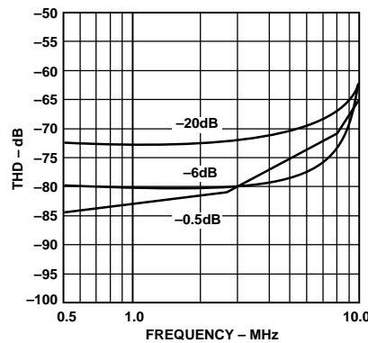
Figure 24. THD vs. Input Frequency (Input Span = 2.0 V p-p, V_{\text{CM}} = 2.5 \text{ V} )
