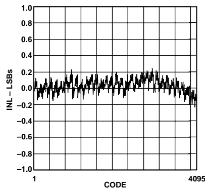
Figure 21. Typical INL
