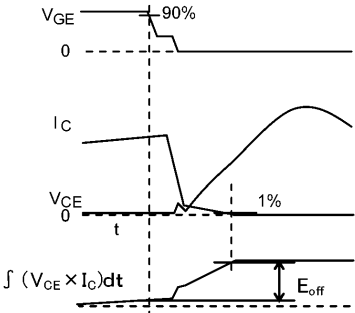
Fig. 6.2.4 Timing Chart of Switching Loss
