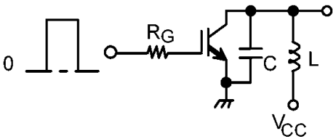
Fig. 6.2.3 Test Circuit of Switching Loss
