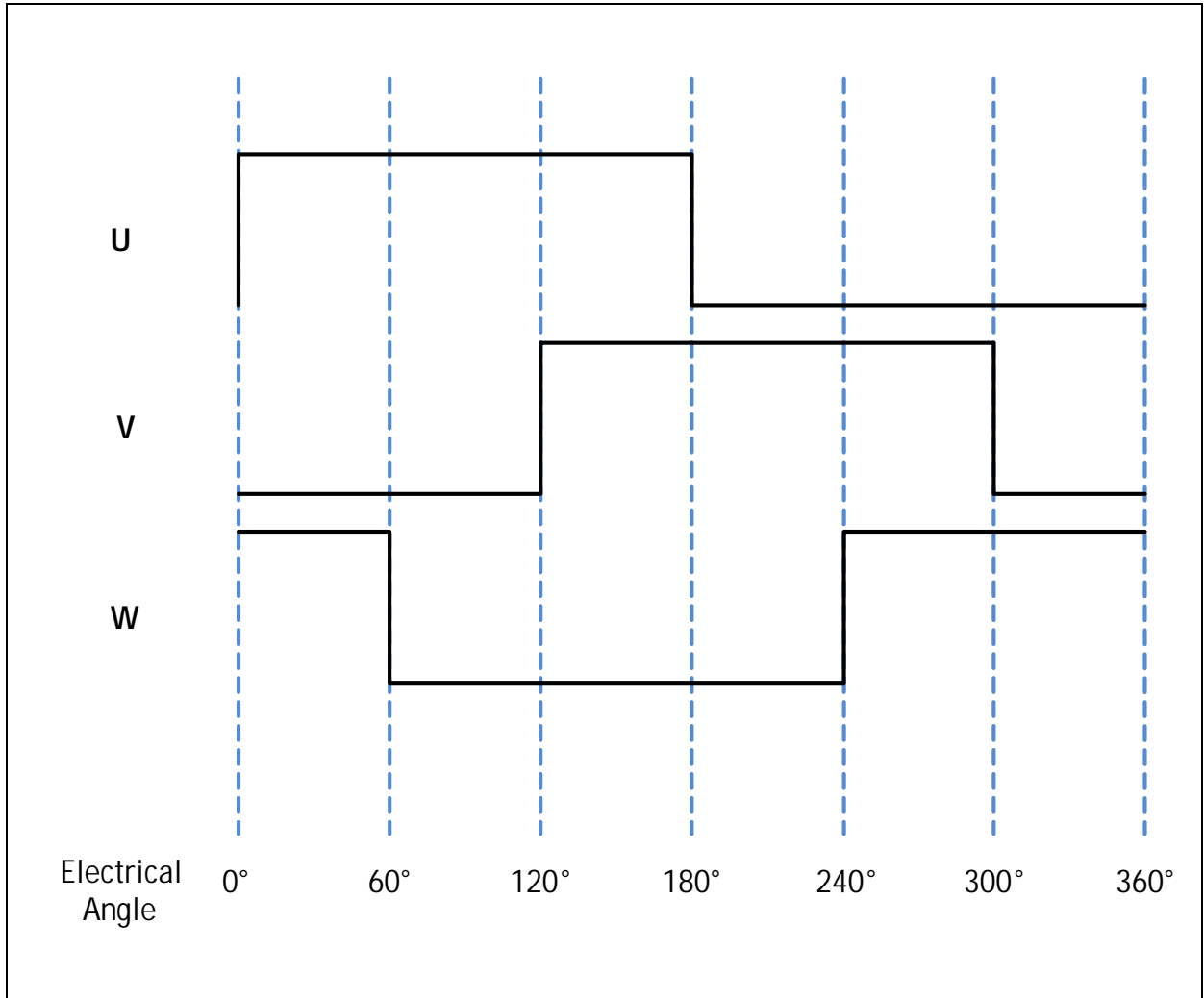
Figure 33 shows the UVW signals for a magnet rotating clockwise, as viewed from above the magnet and the AS5147P. The (DIR=0) bit can be used to invert the sense of the rotation direction.
