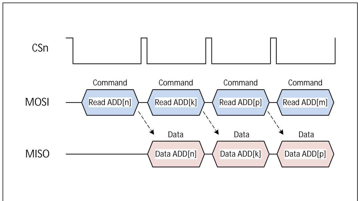
Figure 16: SPI Read
