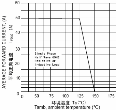
FIG. 3 – 反向特性曲线(典型) FIG. 3 – TYPICAL REVERSE CHARACTERISTICS
