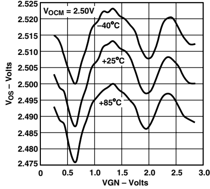
TPC 11. Output Offset vs. VGN
