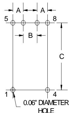
Board Layout
