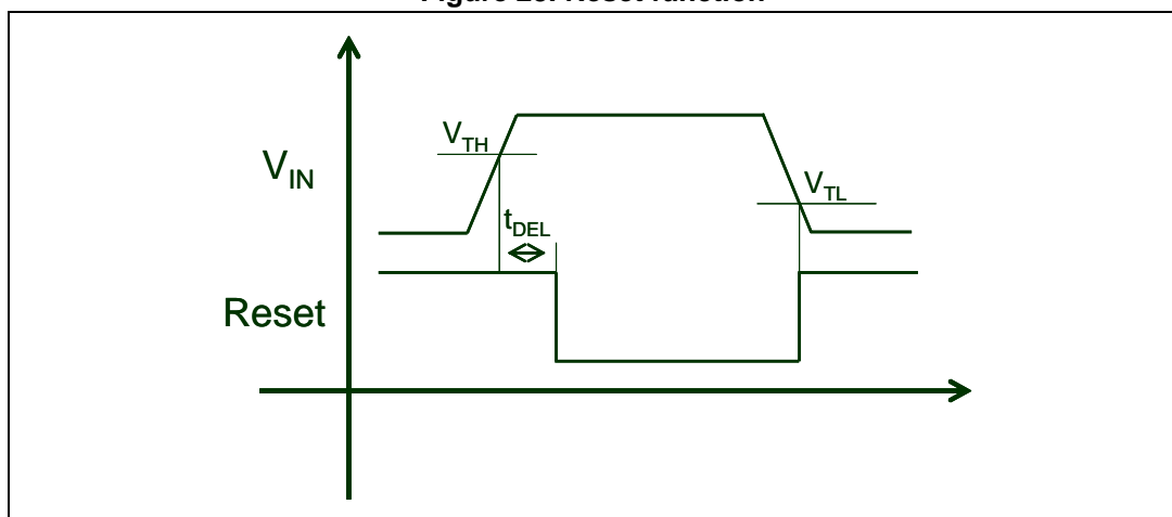
Figure 23. Reset function
